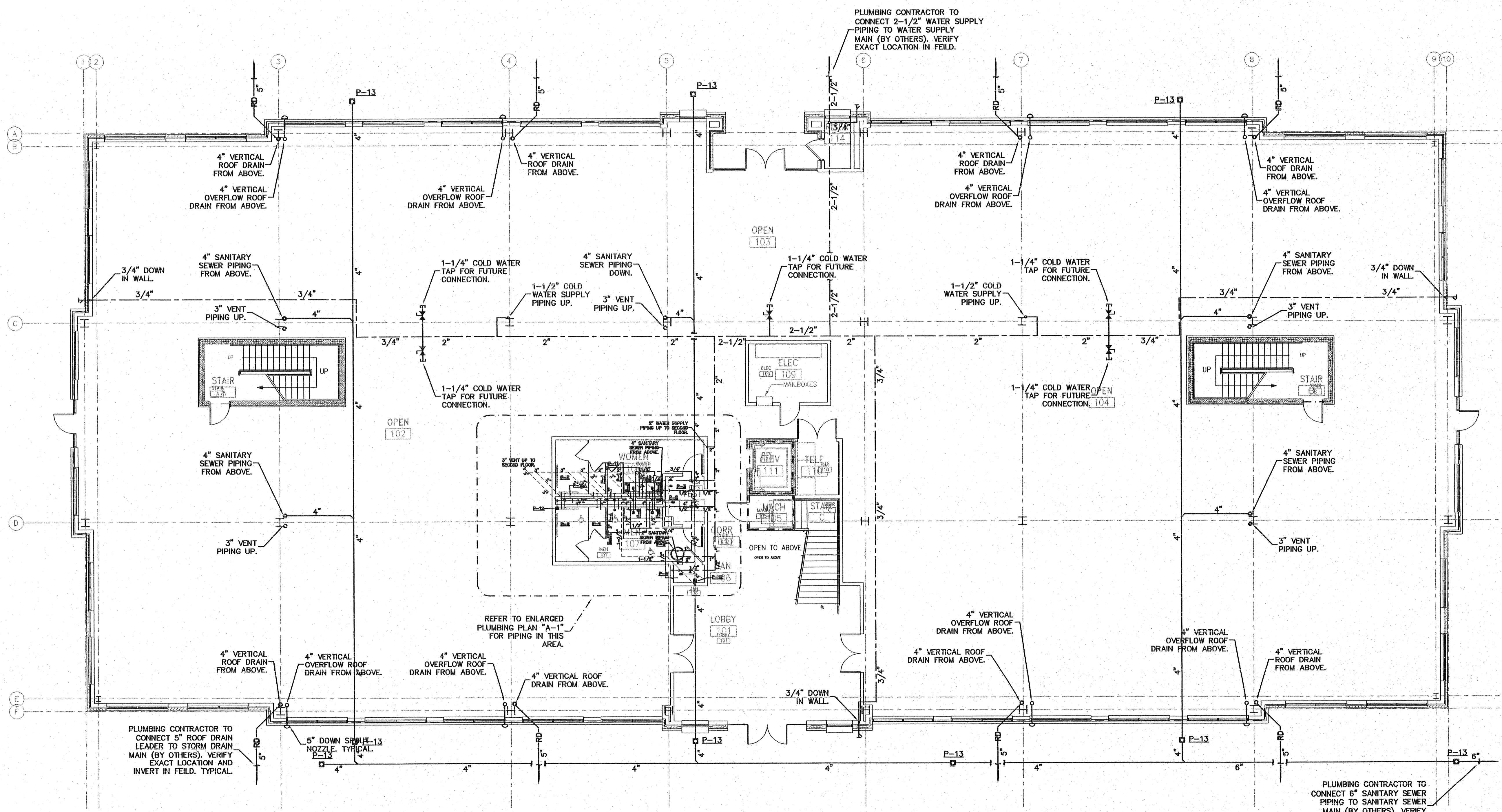
OVERALL FIRST FLOOR PLUMBING PLAN SCALE: 1/8" = 1' - 0"
