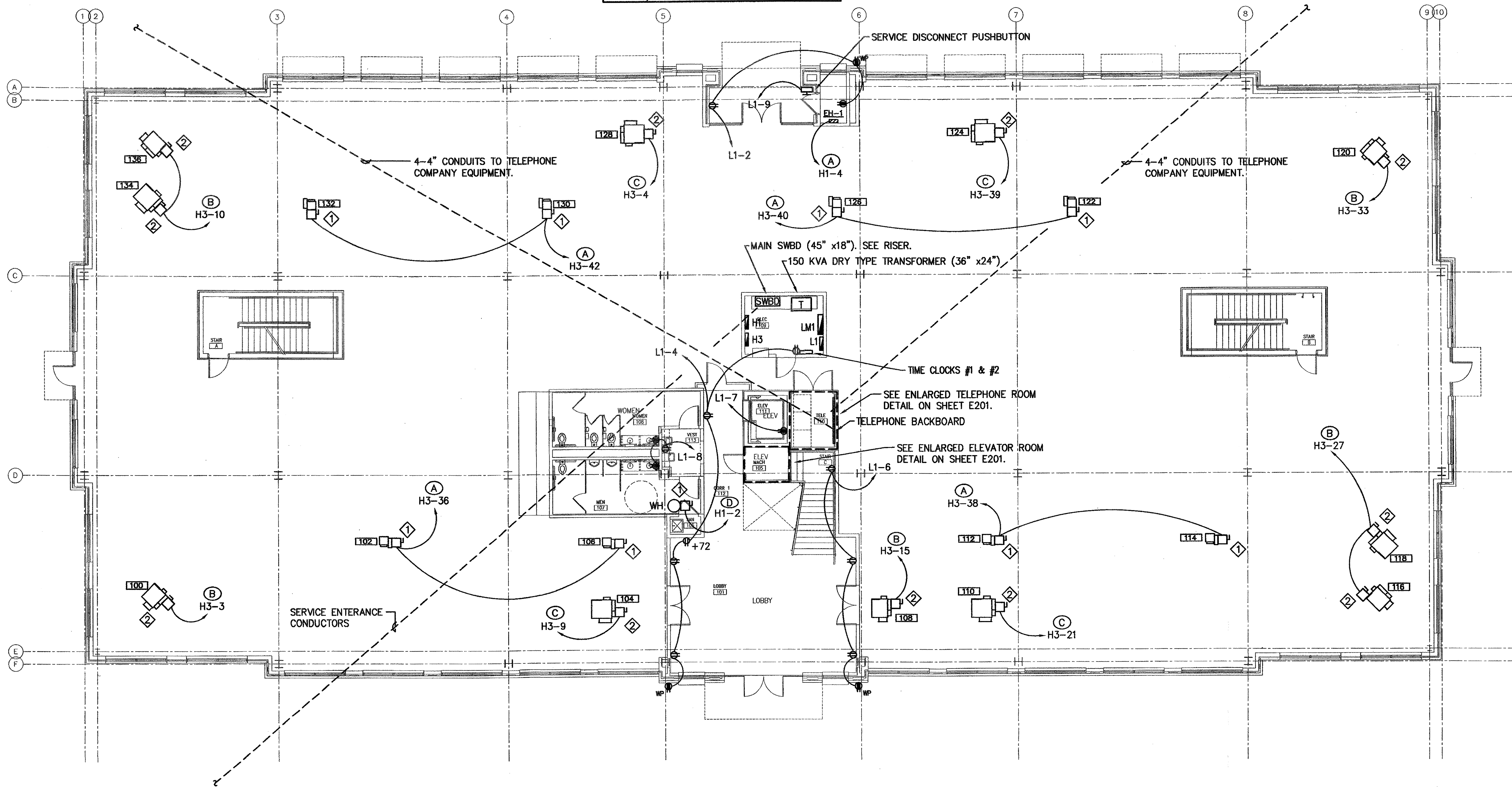
FIRST FLOOR POWER PLAN SCALE: 1/8"=1'-0"
