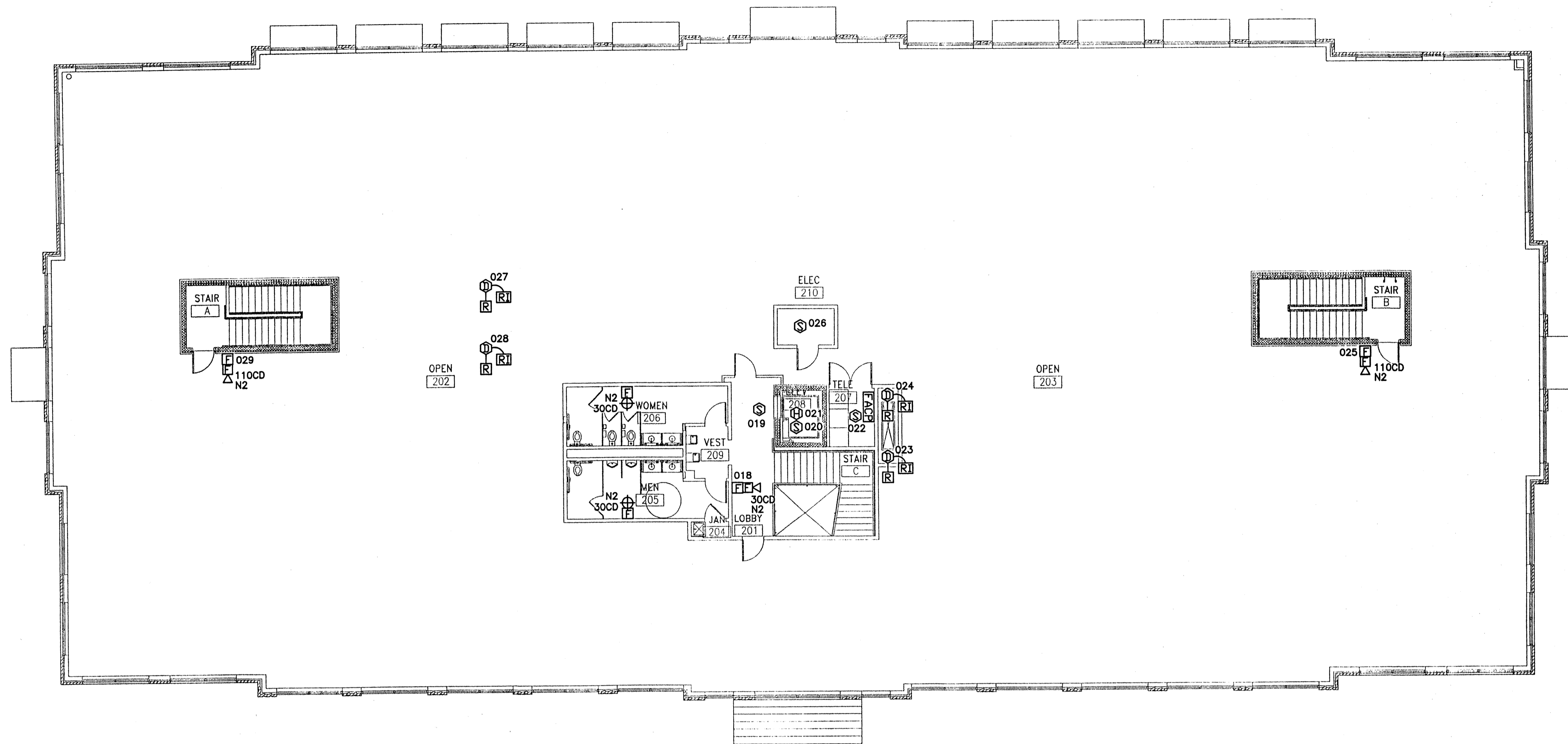
FIRE ALARM SYSTEM - SECOND FLOOR PLAN SCALE: 3/32" = 1'-0"
