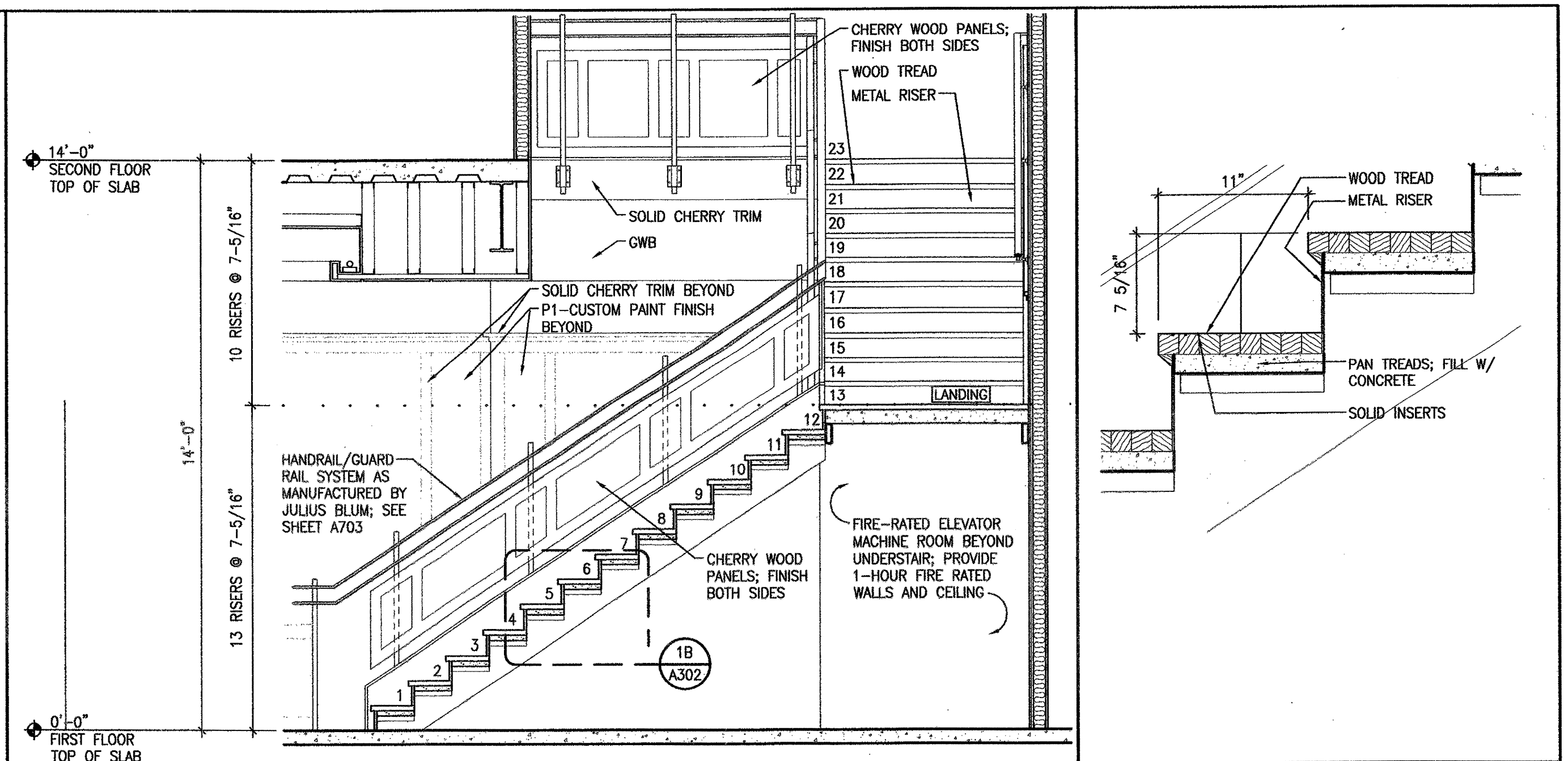
1A SECTION 1B DETAIL 3/8"=1'-0" @ STAIR C 1 1/2"=1'-0" @ STAIR C
