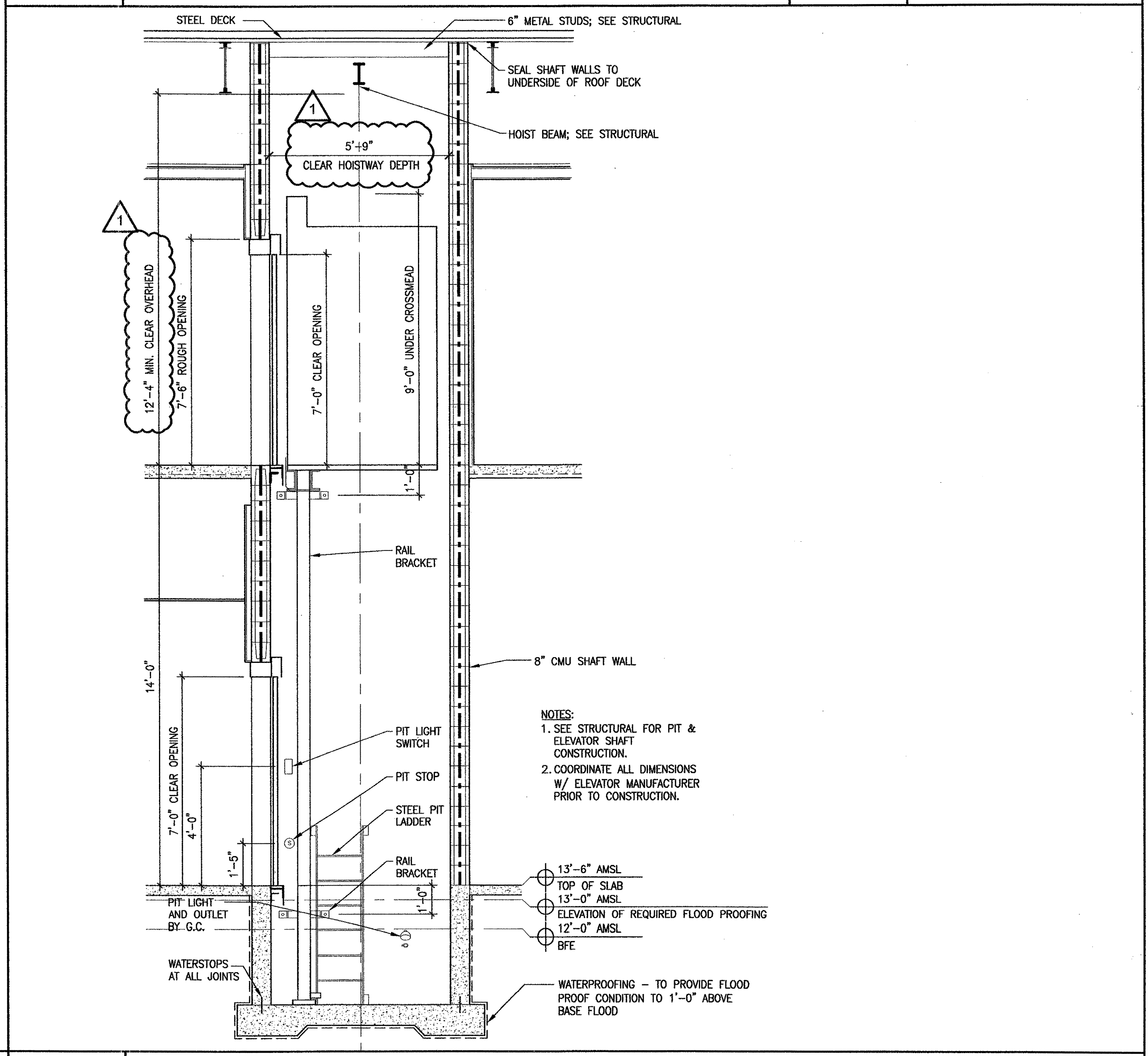
2 SECTION 3/8"=1'-0" @ ELEVATOR SHAFT
