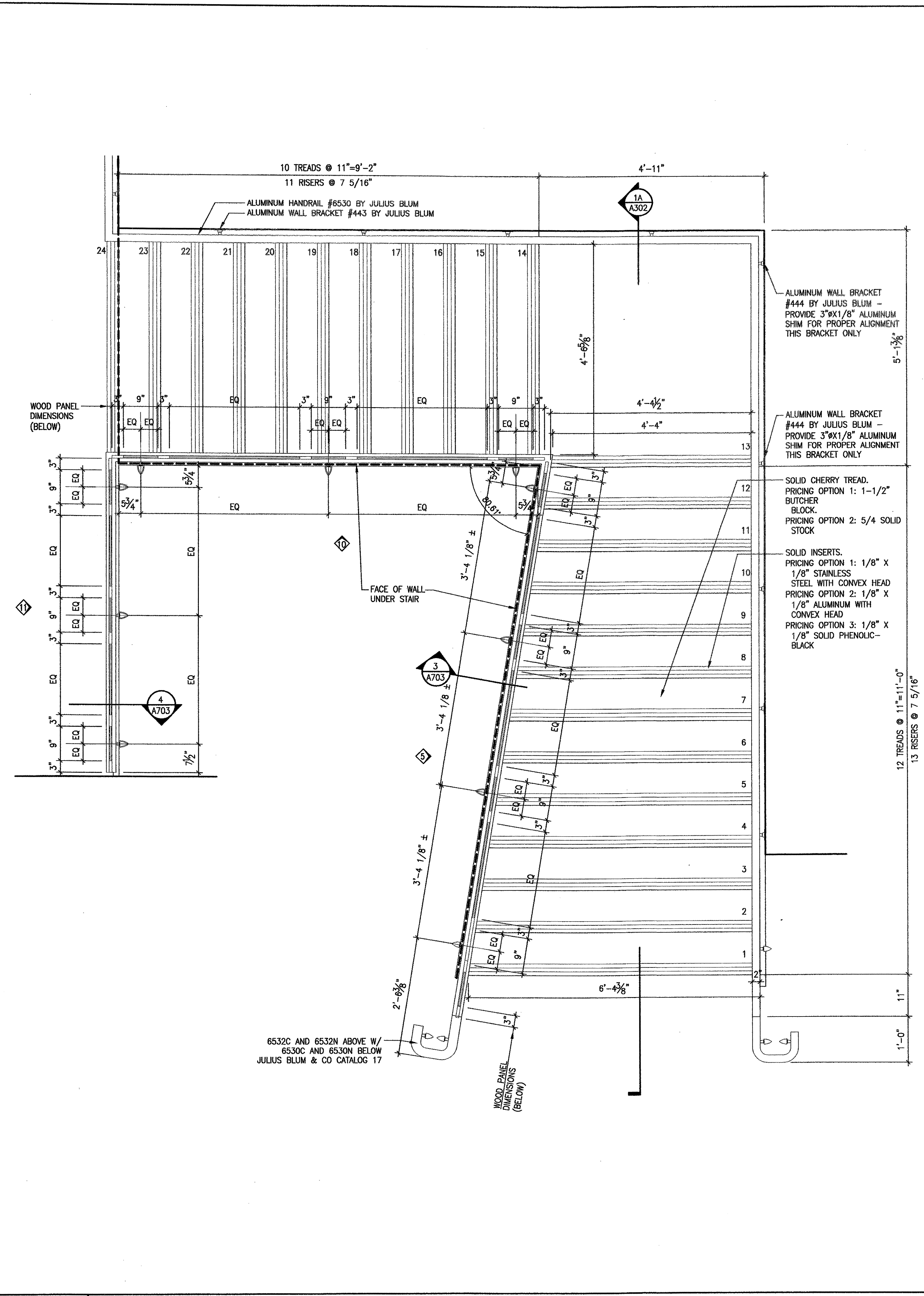
1 STAIR C ENLARGED PLAN 3/4"=1'-0"
